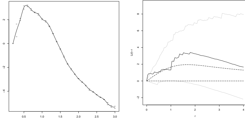
Figure 12: Fitting a shot noise Cox process model to the North Atlantic whales data set. Left: profile log likelihood function l_p(\omega) = \max_{(\kappa, \alpha)} \log L(\theta) obtained by cumulating estimated log likelihood ratios, see text. The small horizontal bars indicate 95% Monte Carlo confidence intervals for the log likelihood ratios. Right: non-parametric estimate of L(r) - r (solid line), 95% confidence envelopes based on simulations of fitted shot noise Cox process (dotted lines), L(r) - r = 0 for a Poisson process (lower dashed line), and L(r) - r > 0 for the fitted shot noise Cox process (upper dashed line).
