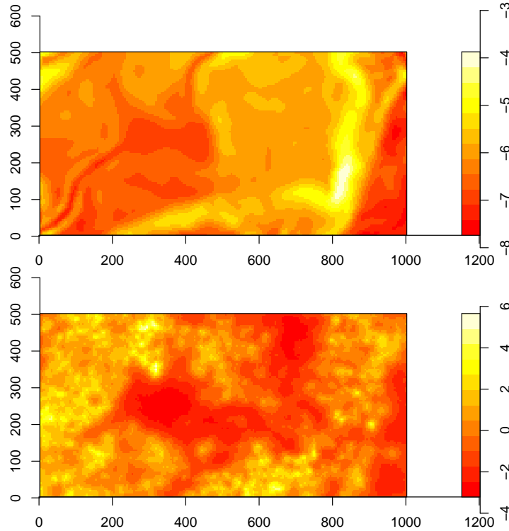
Figure 13: Posterior mean of \beta_1 + \beta_2 z_2(u) + \beta_3 z_3(u) (upper) and \Psi(u) (lower), u \in W , under the log Gaussian Cox process model for the tropical rain forest trees.
