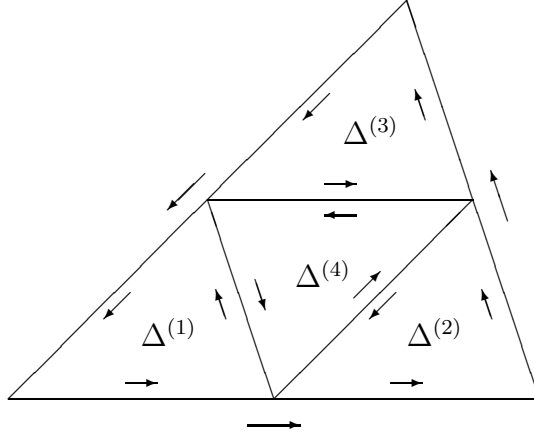
Figure 1: Partition of \Delta .
