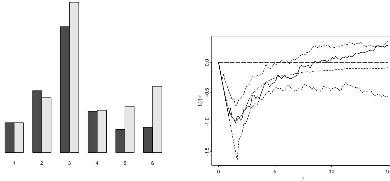
Figure 11: Model assessment for Norwegian spruces (Example 7.1). Dark grey bars: frequencies of trees for the six size classes (scaled so that light and dark bars are of the same height for the first class). Light gray bars: MLE of \exp(\beta_k) , k = 1, \dots, 6 . Right plot: estimated L(r) - r function for spruces (solid line) and average and 95% envelopes computed from simulations of fitted overlap interaction model (dashed lines).
