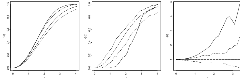
Figure 10: Left to right: estimated F , G , and J -functions for the Norwegian spruces (solid lines) and 95% envelopes calculated from simulations of a homogeneous Poisson process (dashed lines) with expected number of points equal to the observed number of points. The long-dashed curves show the theoretical values of F , G , and J for a Poisson process.
