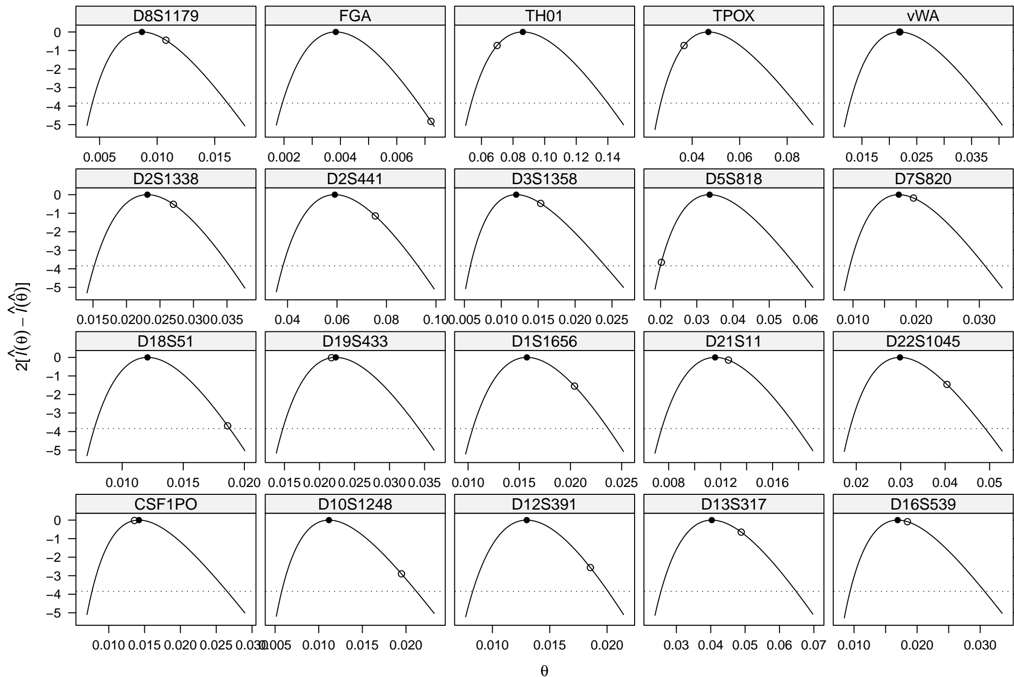
\theta -estimates based on data from 7 major population groups
