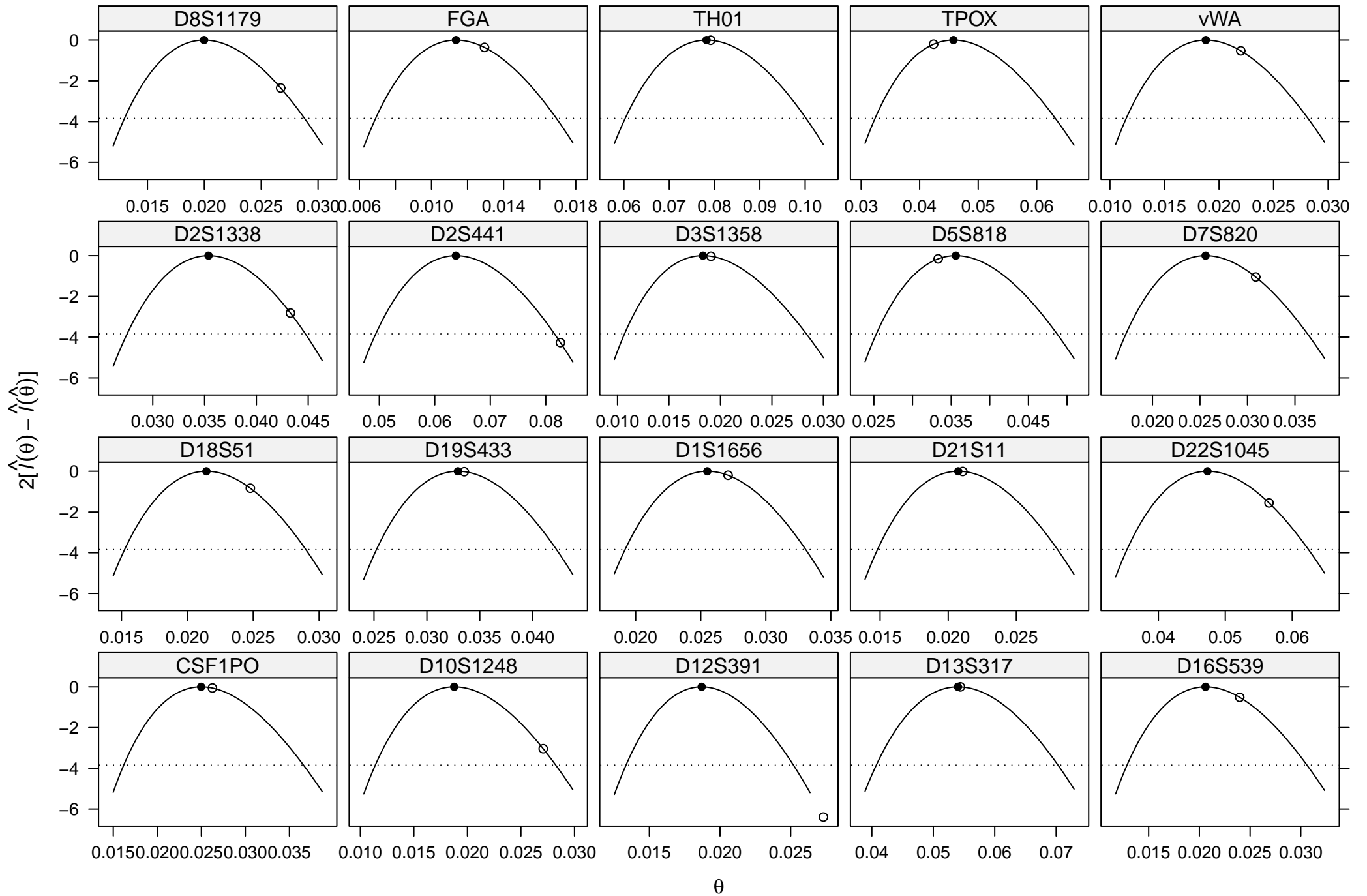
\theta -estimates based on data from 51 populations
